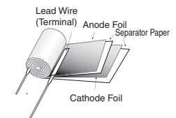
Winding Model
